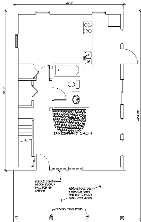
1 EXISTING PLAN Scale: 1/4" = 1'-0"
