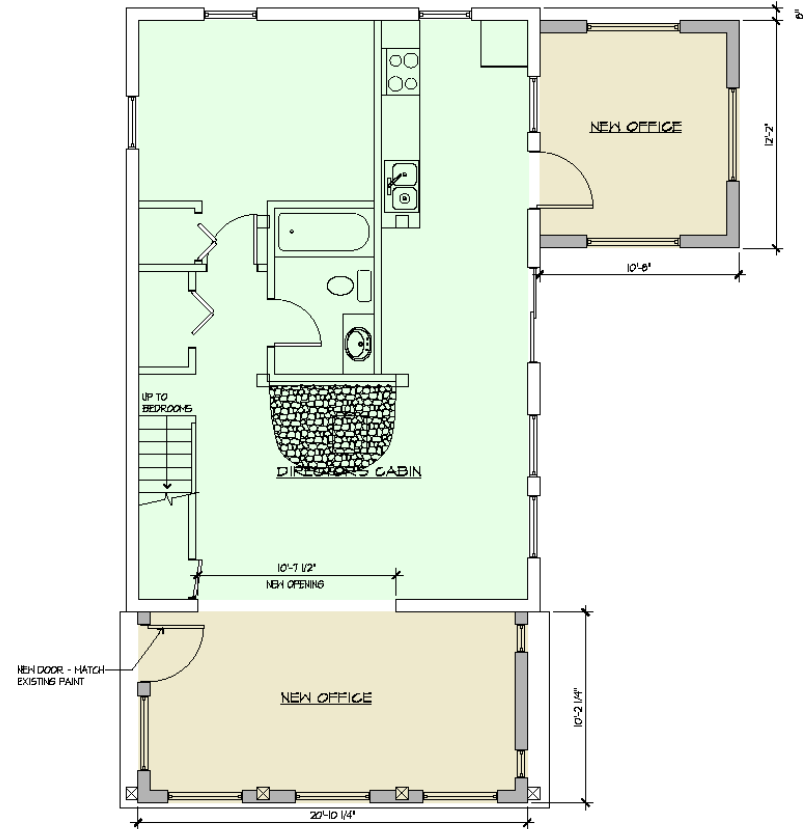
2 ADDITION PLAN Scale: 1/4" = 1'-0"
