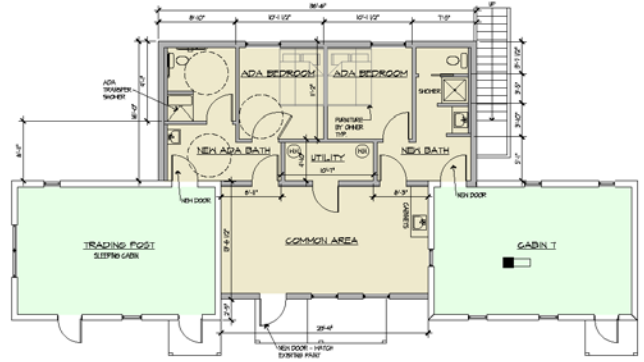
2 A1.0 ADDITION PLAN Scale: 3/8" = 1'-0"
