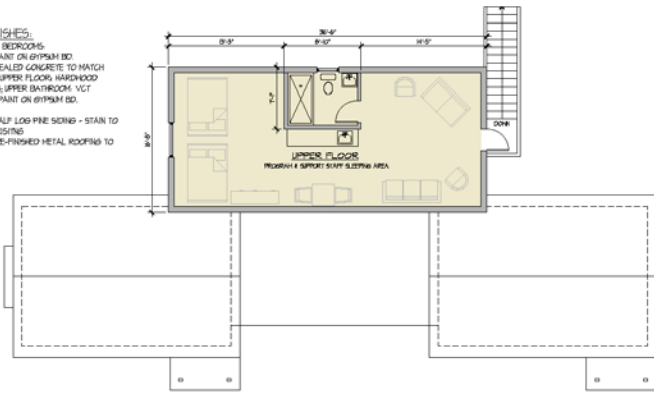
4 A1.0 ADDITION PLAN - UPPER FLOOR Scale: 3/8" = 1'-0"
